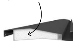
Louwer structure Sandwich construction with Peripor core.
