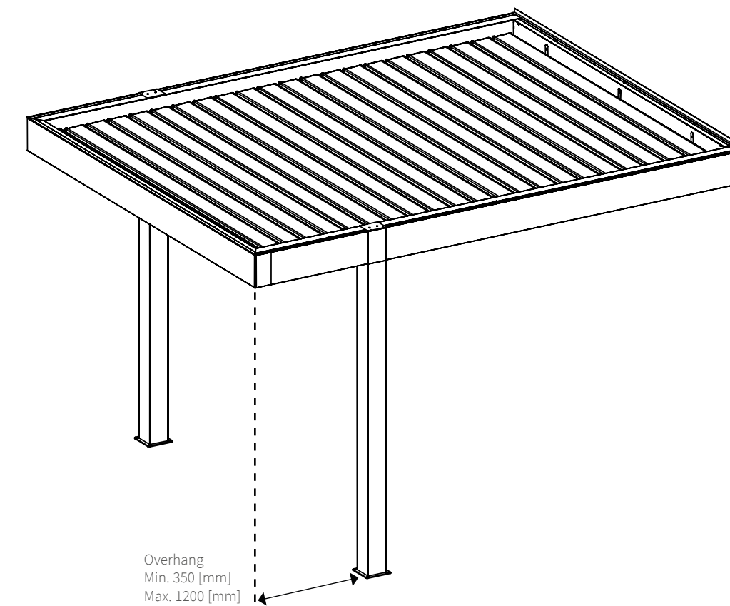
V870 - Arezzo | Type with overhang
